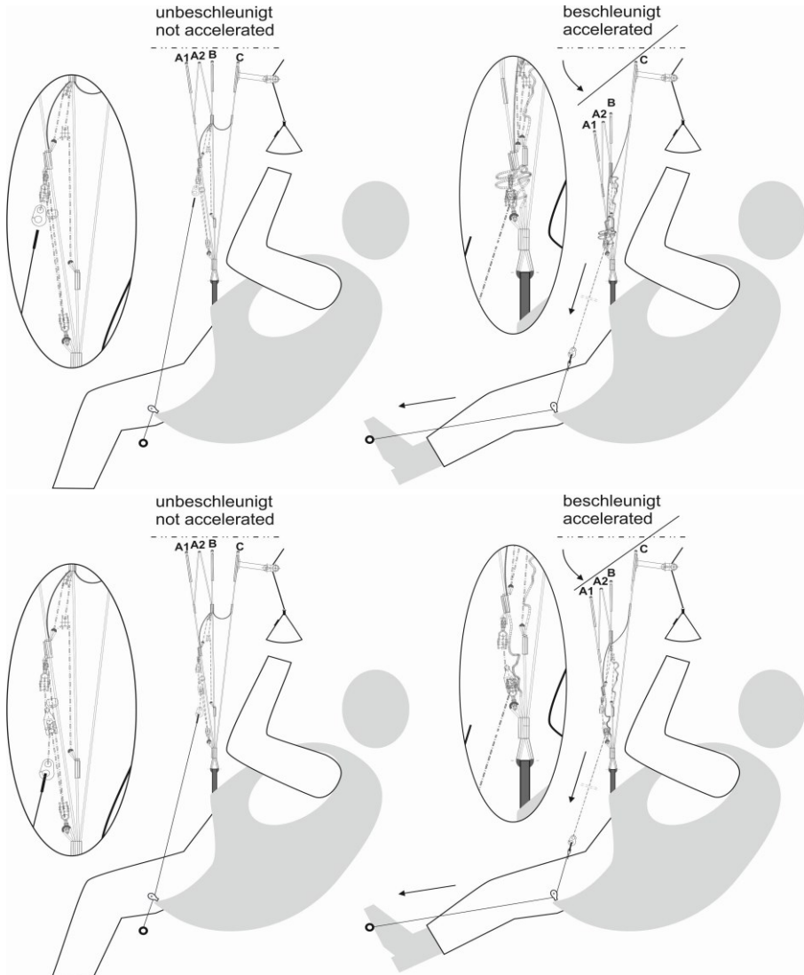
Fig. 7 How the MIURA 2 RS speed system works (MIURA 2 RS without speed limiter top figure, MIURA 2 RSe with speed limiter bottom figure)
