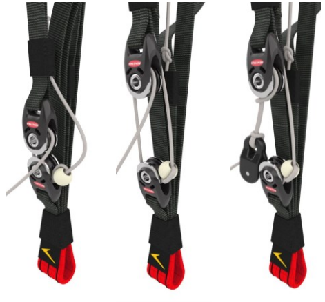
Fig. 8 MIURA 2 RS riser at speed steps with and without speed limiter
